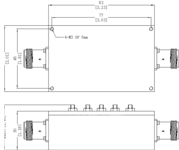
N-Type 50 Ohm
